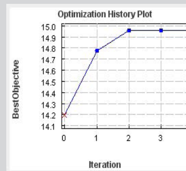
Analysis on the Optimized Wing Shape using ANSYS Fluent
