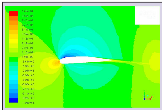
Analysis on the Optimized Wing Shape using ANSYS Fluent
